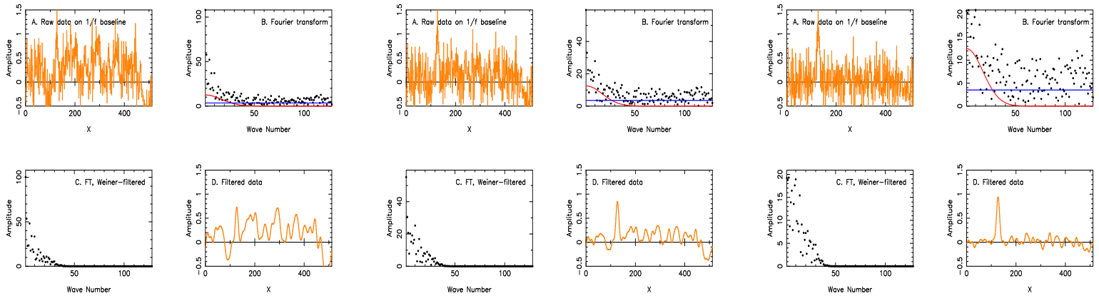
Figure 1: Starting with the raw data of Figure 8.1, a baseline created from random Gaussian noise filtered by 1/f has been added in proportions (left-to-right plot-sets) 10:5:1. The Wiener filtering of the example has been left untouched.
